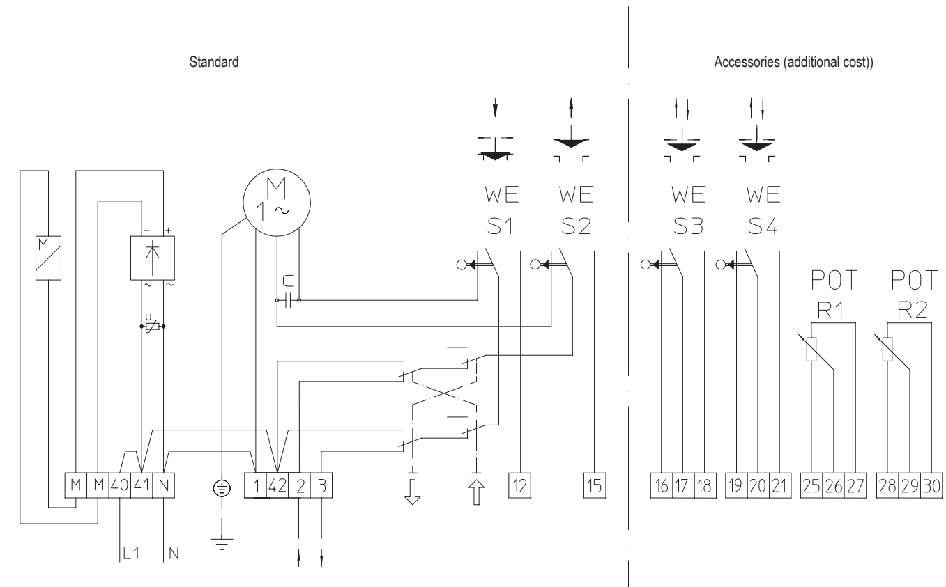
Wiring diagram FR 2.1 and FR 2.2
