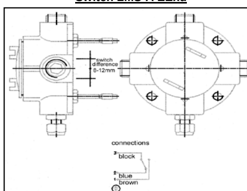
Switch LMS-A-EExd
