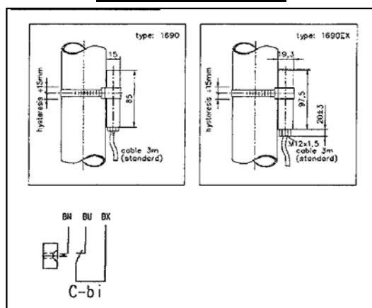
Switch 1690 / 1690ATEX
