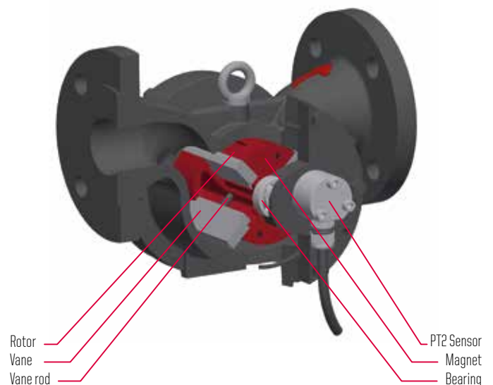
Section view of a PT2 Flowmeter
